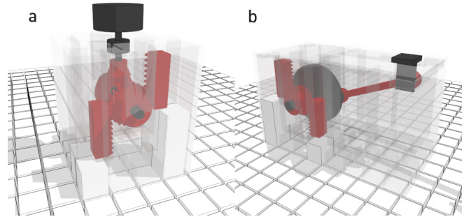
Figure 8. a) Inside view of Rotator 's mechanical system. Two linear gears are driven by the pins which translates into rotation using a gear train b) Gears and a lever create horizontal movement in the Slider block.
